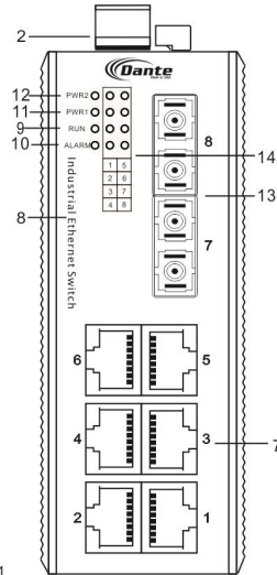
Front panel view
