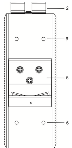
Rear panel view
